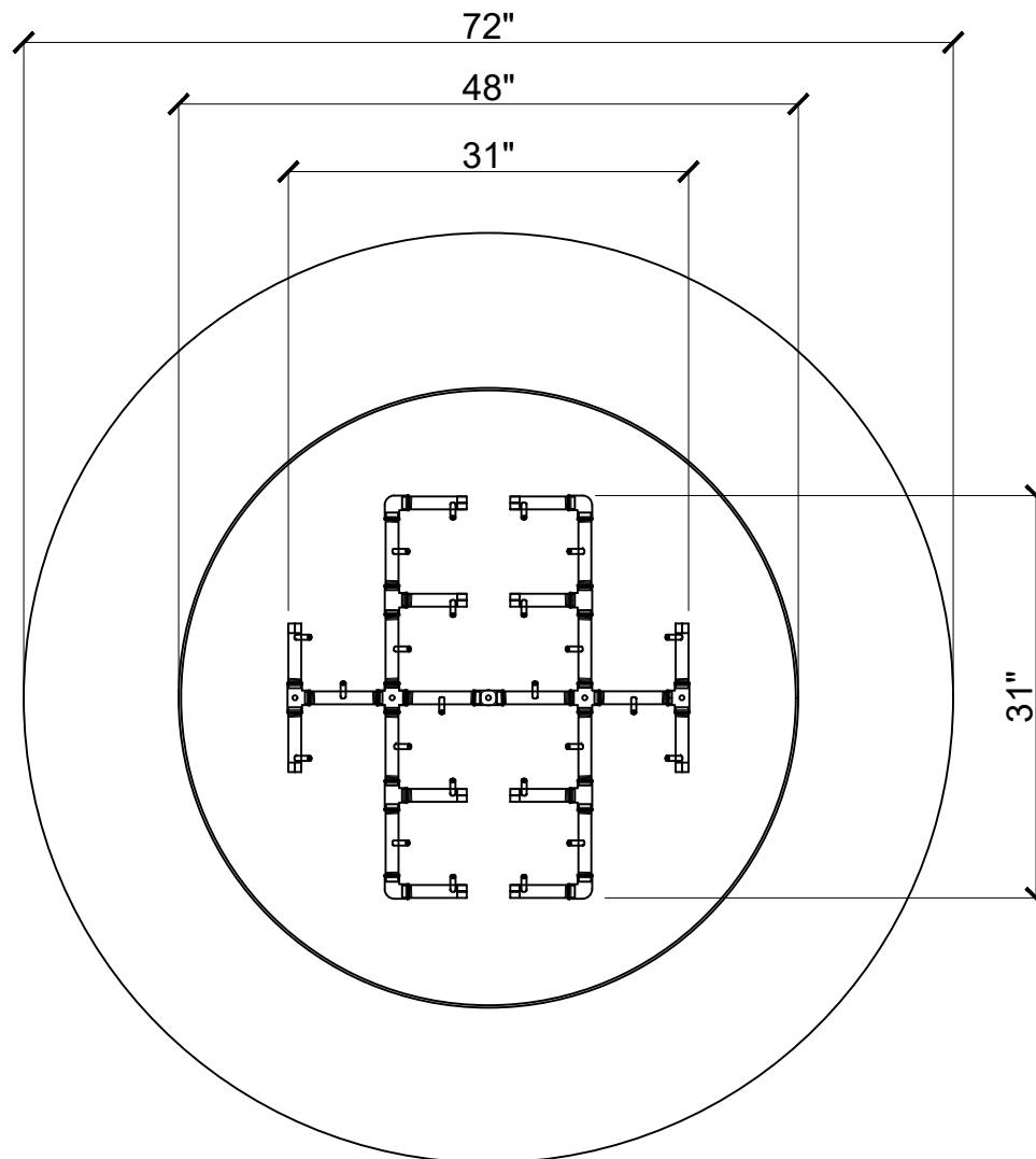
PLAN VIEW
