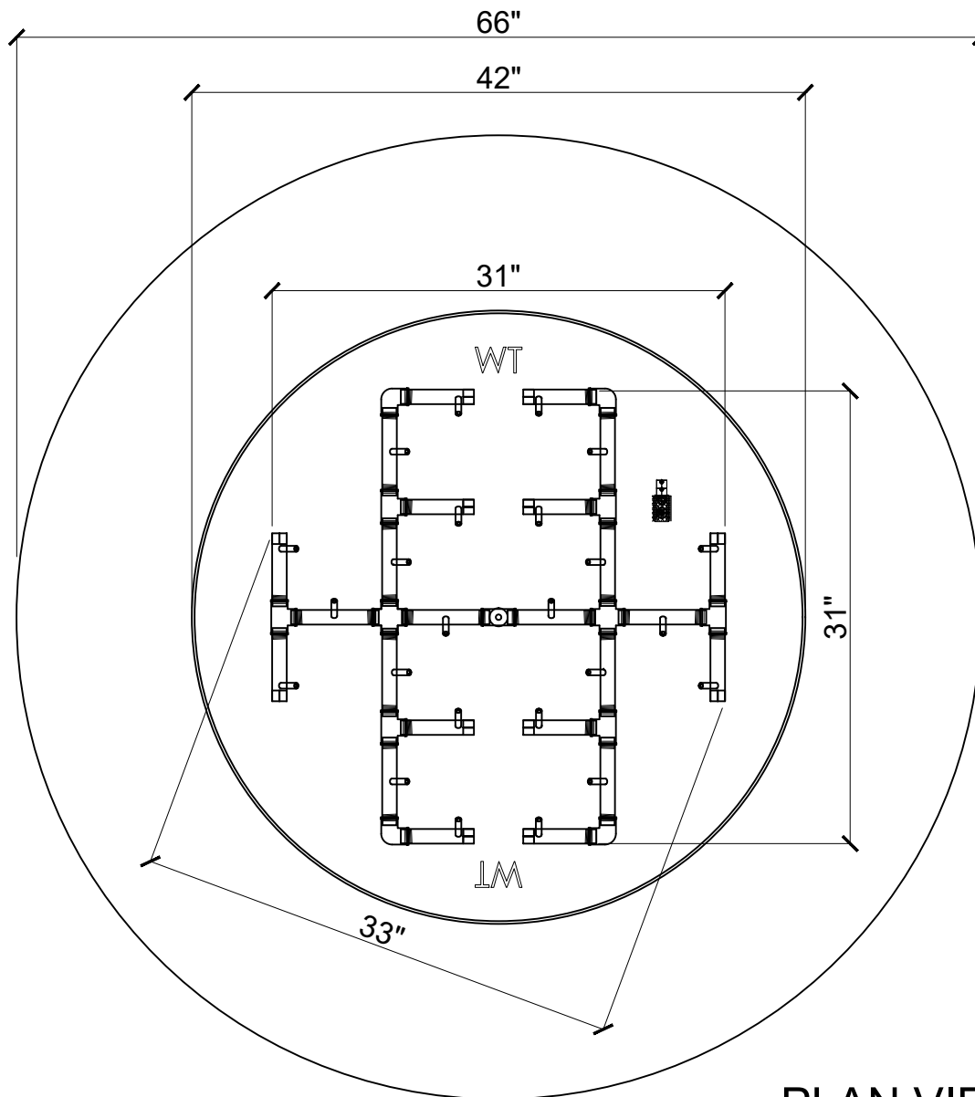
PLAN VIEW
