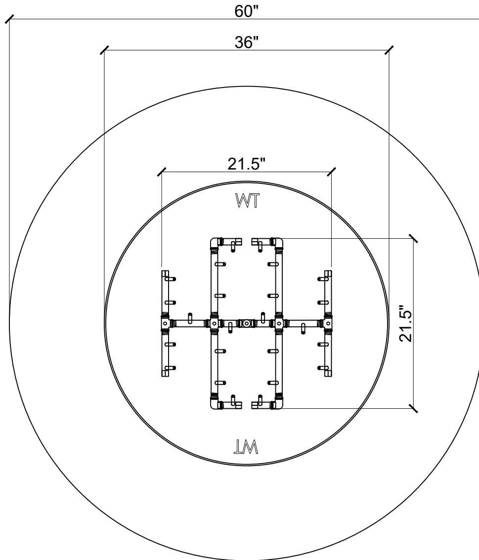
PLAN VIEW
