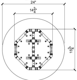
CFBO180 Octagonal CROSSFIRE™ Brass Burner
