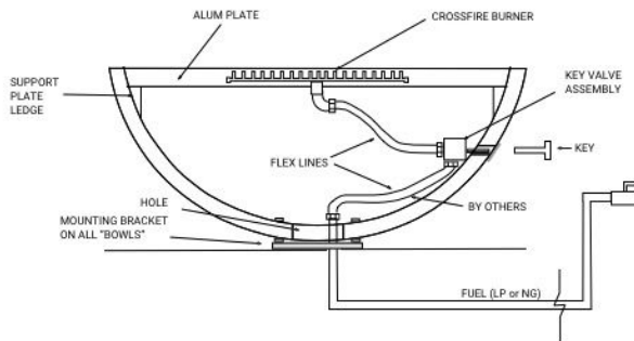
CFBO180 Octagonal CROSSFIRE™ Brass Burner
