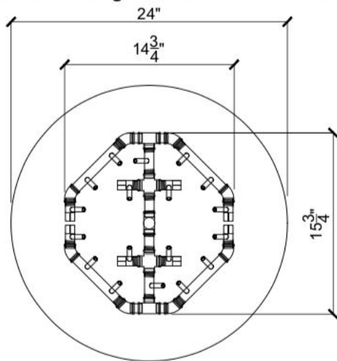
PLAN VIEW
