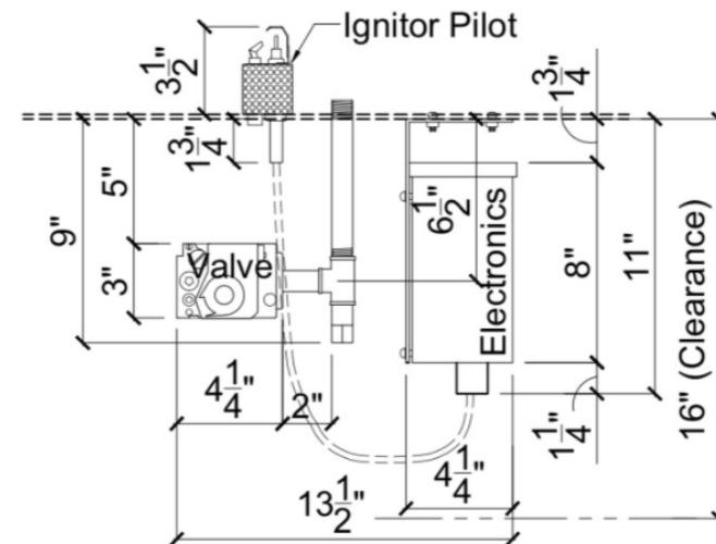
SIDE ELEVATION 'C'
