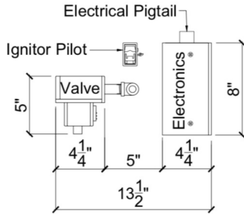
TOP VIEW 'A'
