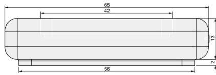
02 FRONT VIEW
