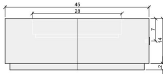
02 FRONT VIEW
