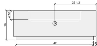
03 SIDE VIEW
