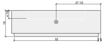
03 SIDE VIEW
