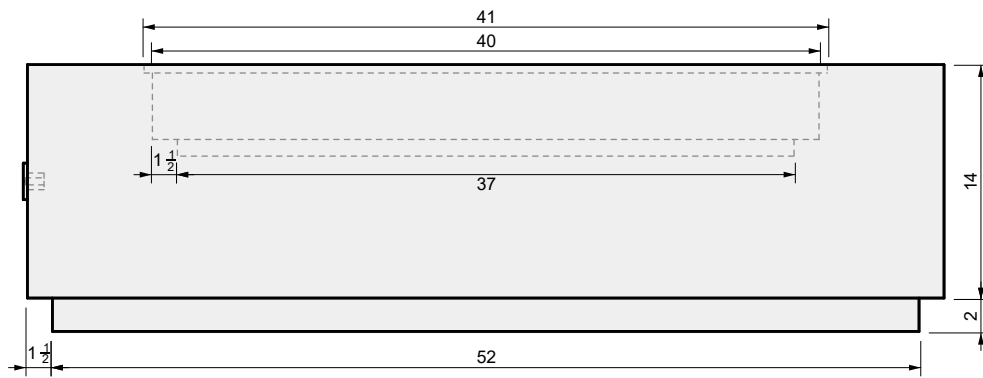
02 FRONT VIEW
