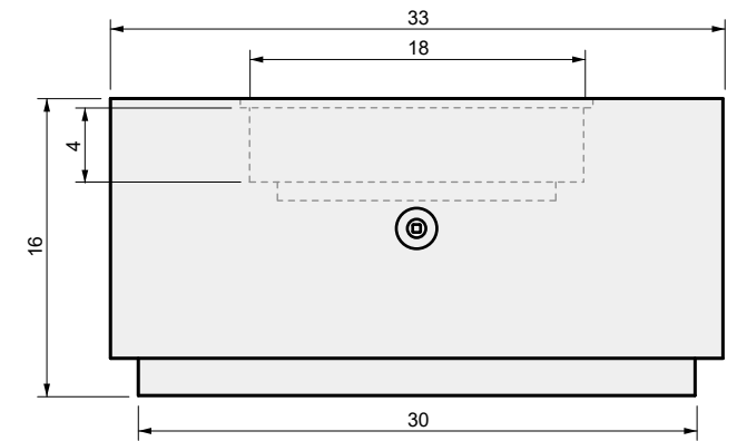
03 SIDE VIEW
