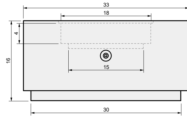
03 SIDE VIEW
