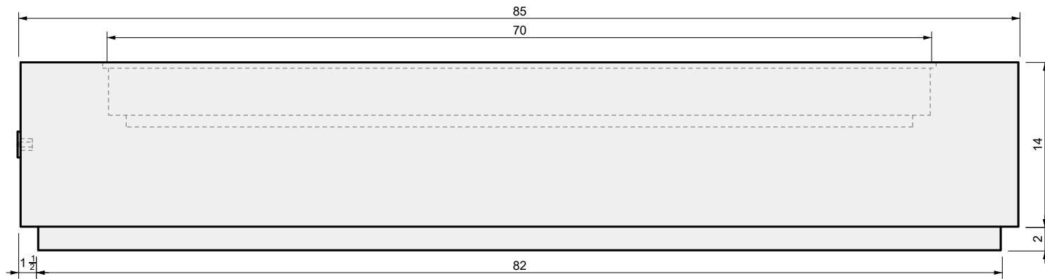
02 FRONT VIEW
