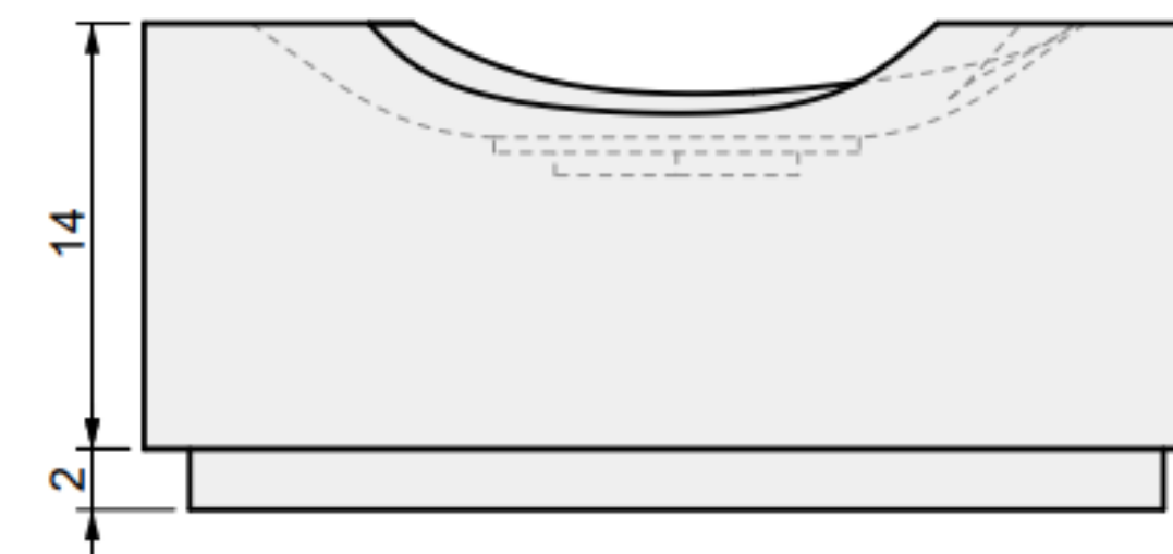
03 SIDE VIEW
