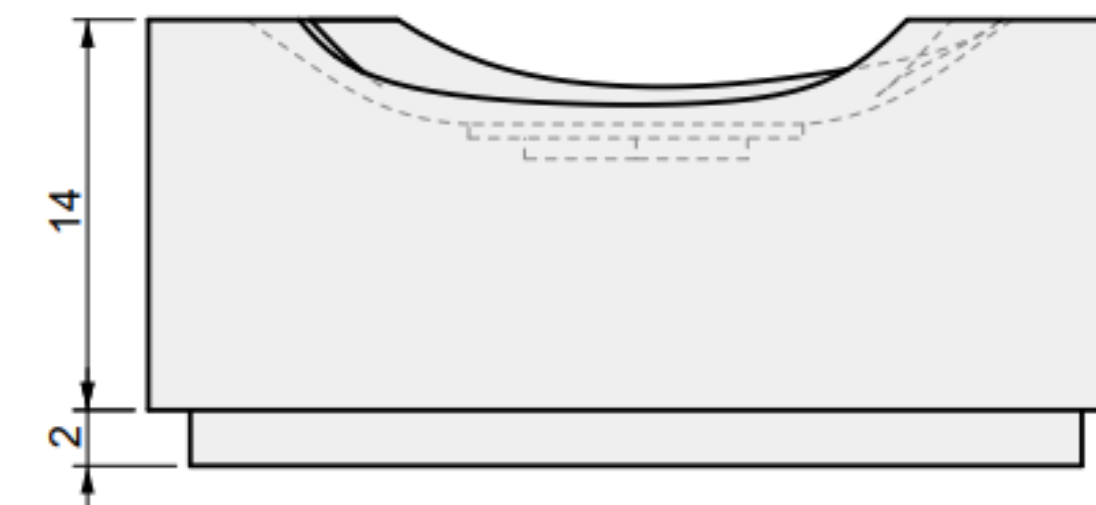
03 SIDE VIEW
