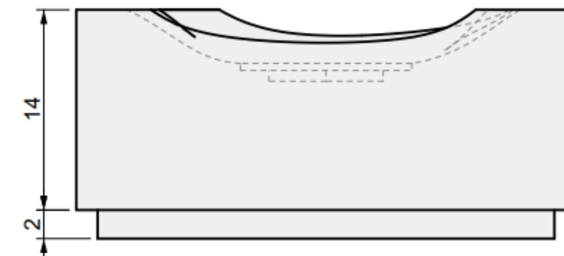
03 SIDE VIEW
