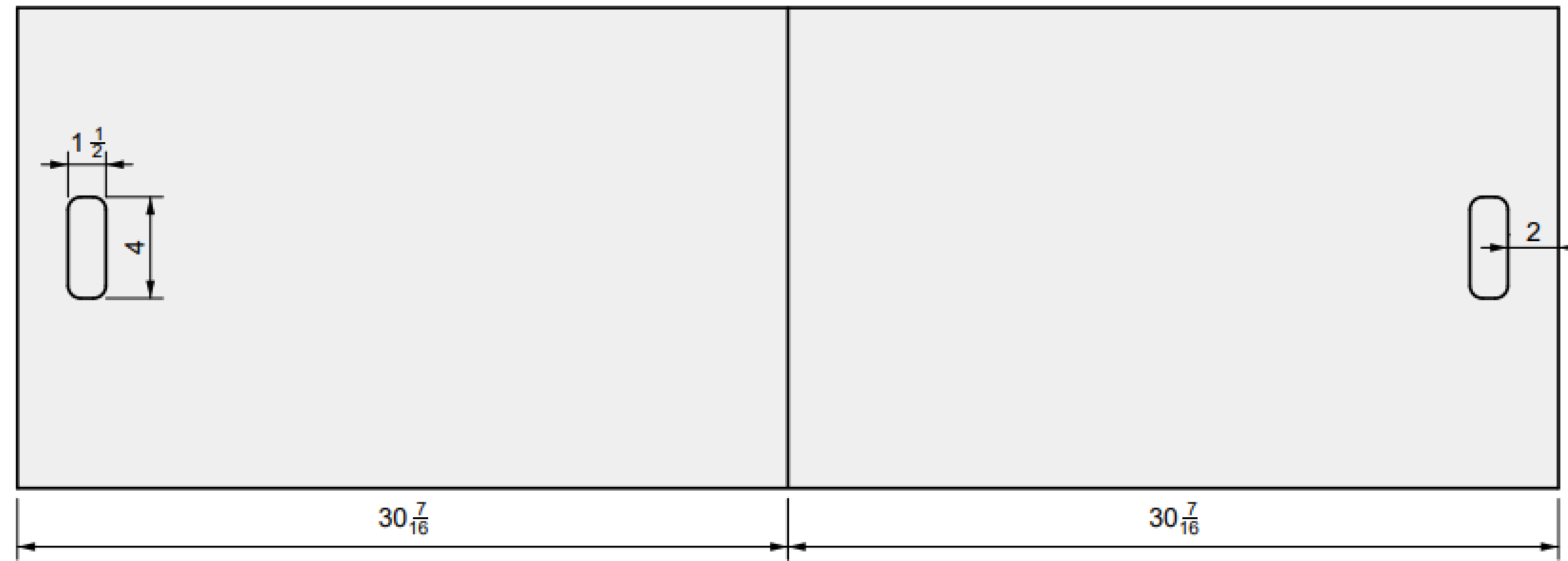
01 TOP VIEW
