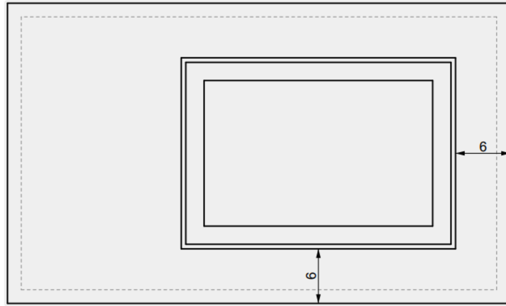
01 TOP VIEW
