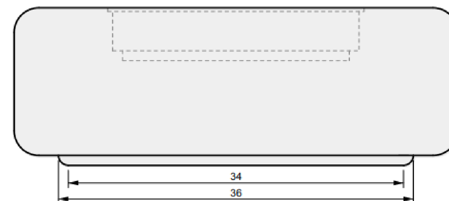
03 SIDE VIEW
