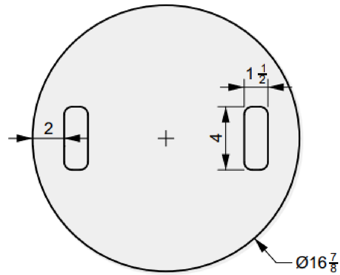
01 TOP VIEW
