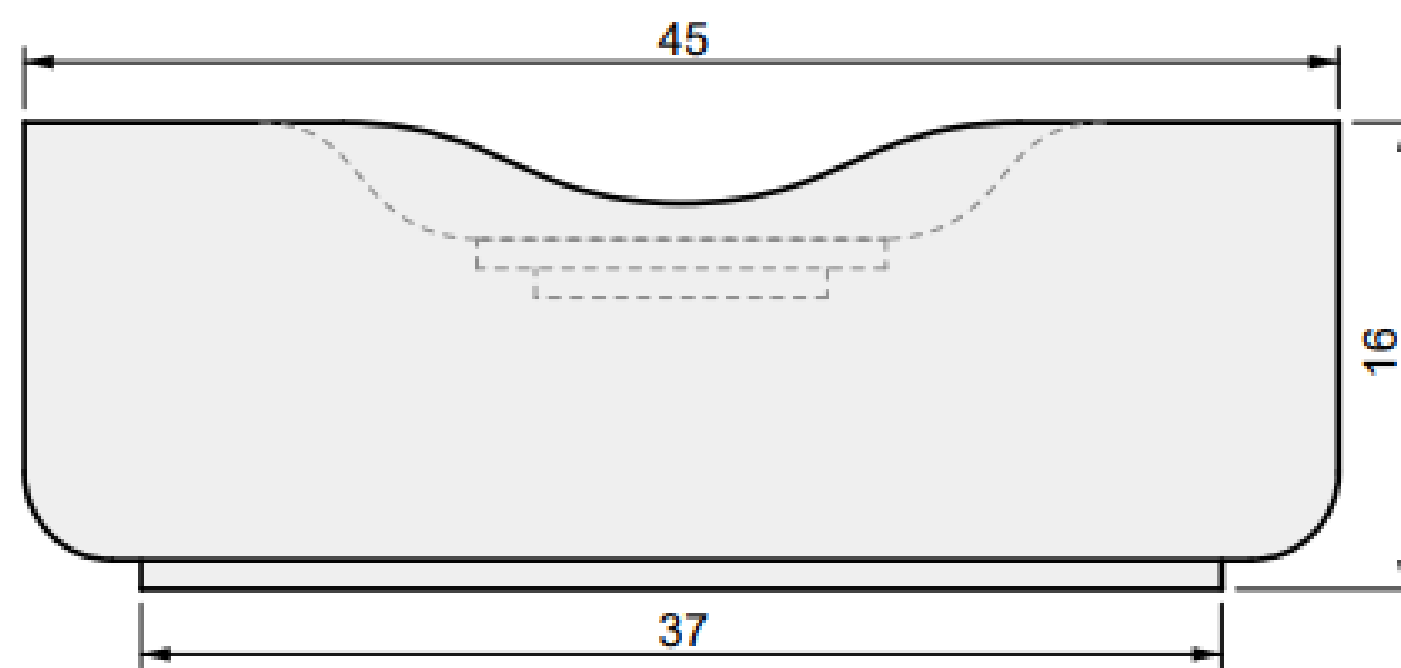
02 FRONT VIEW
