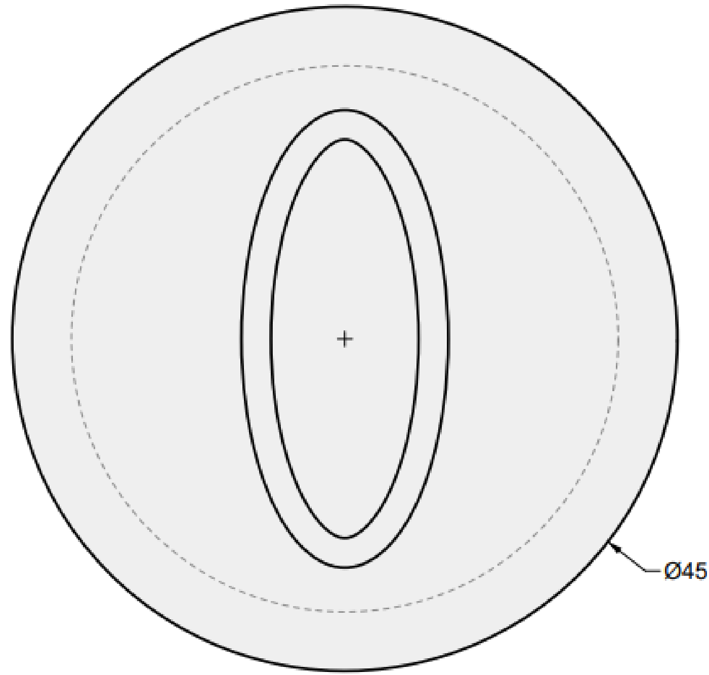
01 TOP VIEW
