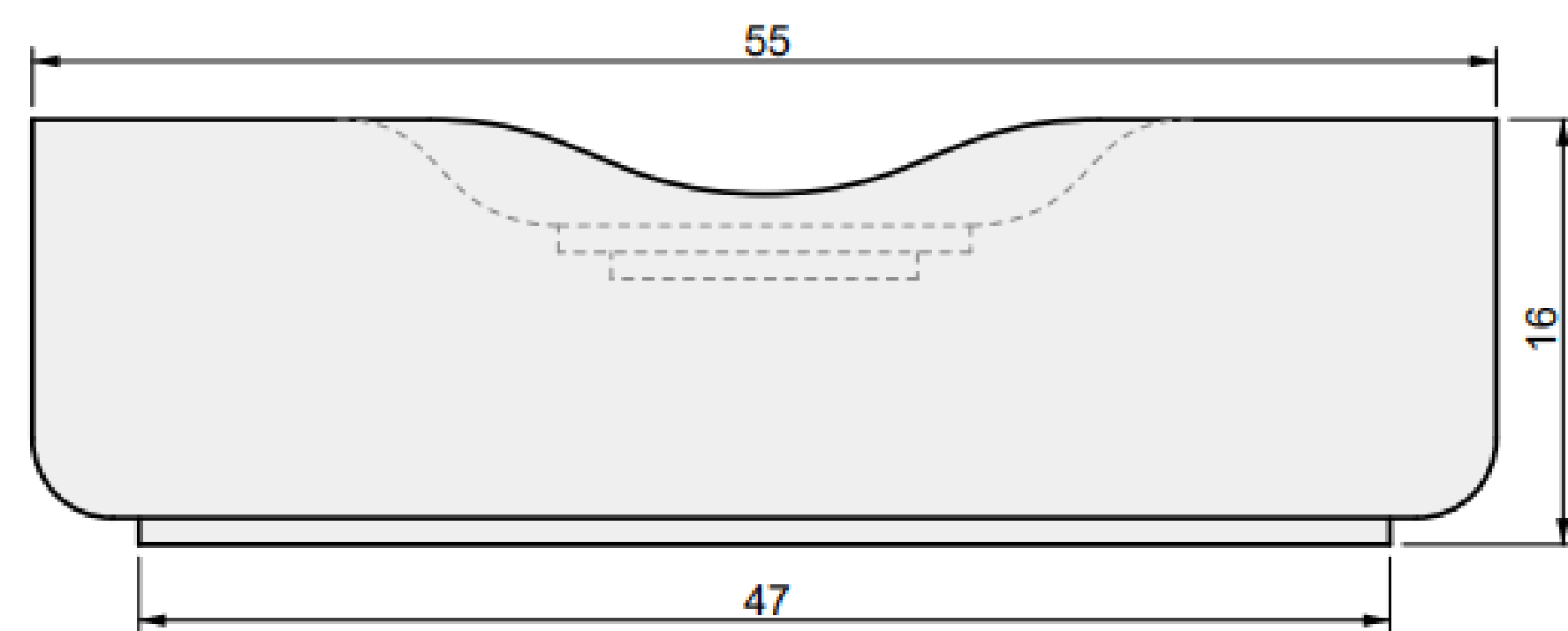
02 FRONT VIEW
