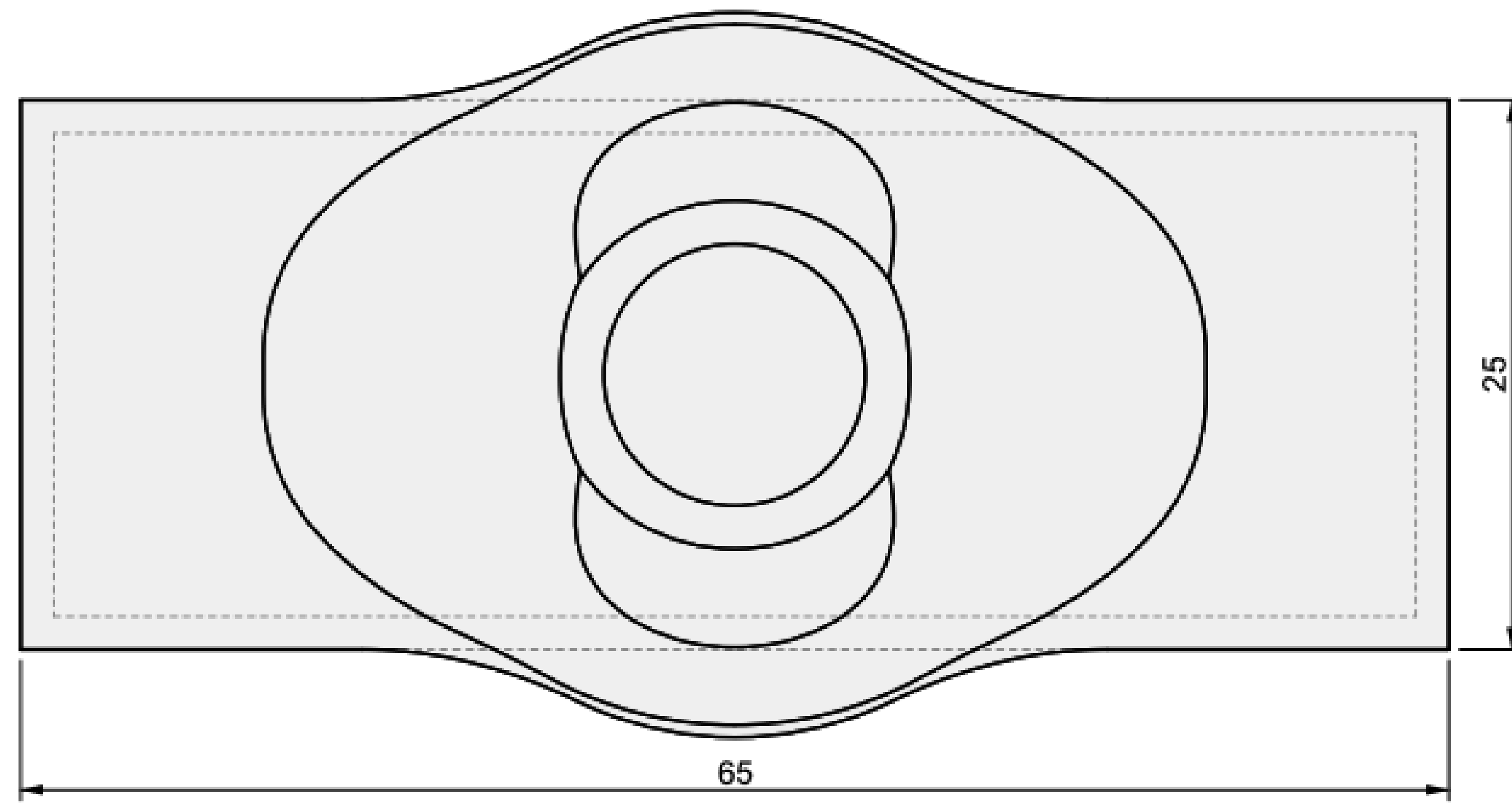
01 TOP VIEW
