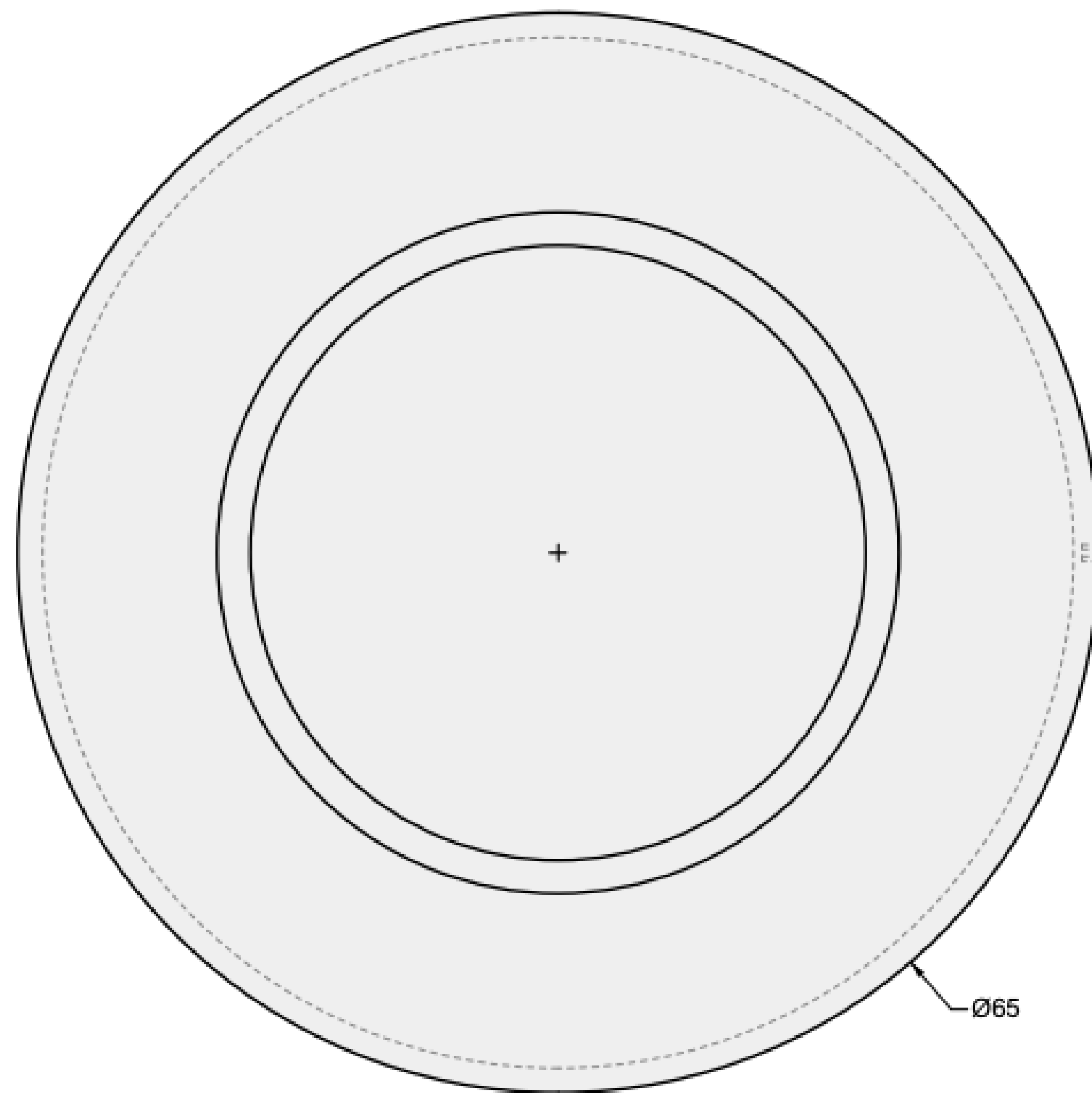
01 TOP VIEW
