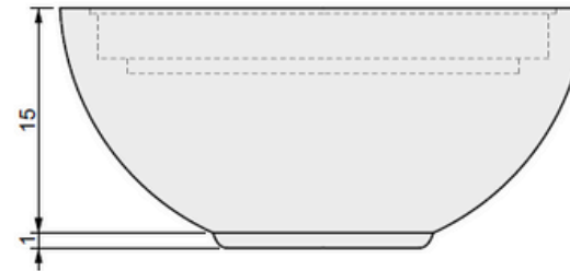
03 SIDE VIEW
