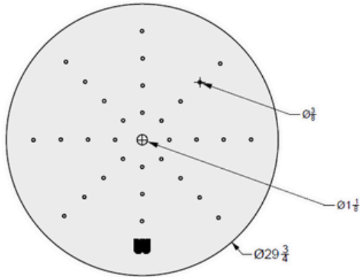
01 TOP VIEW
