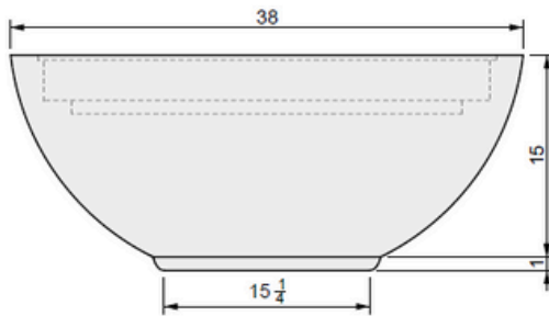
02 FRONT VIEW
