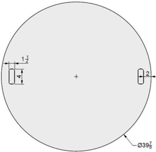
01 TOP VIEW
