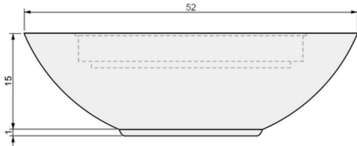
03 SIDE VIEW
