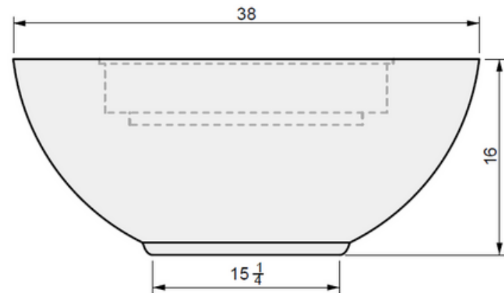
02 FRONT VIEW
