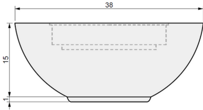
03 SIDE VIEW
