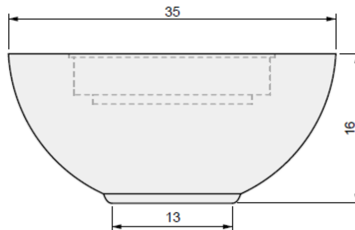
02 FRONT VIEW
