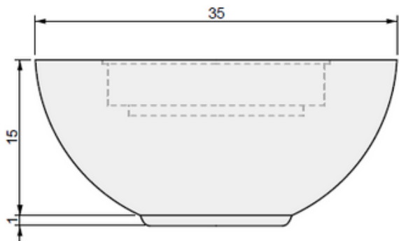
03 SIDE VIEW
