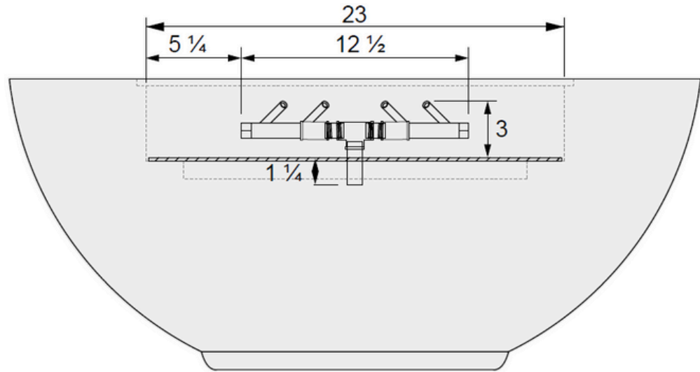
01 SIDE VIEW
