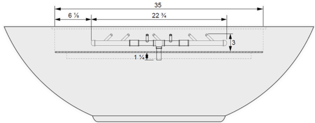
01 SIDE VIEW
