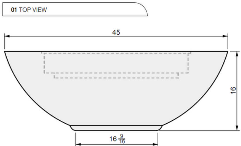
02 FRONT VIEW
