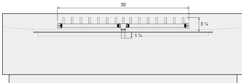
01 SIDE VIEW
