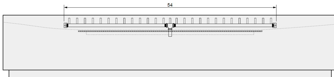
01 SIDE VIEW
