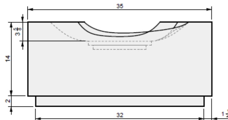
03 SIDE VIEW
