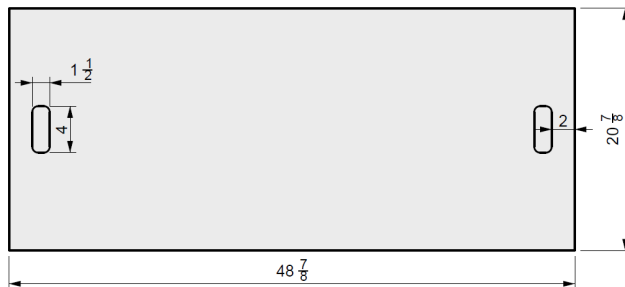
01 TOP VIEW
