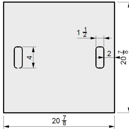
01 TOP VIEW
