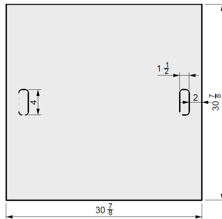
01 TOP VIEW
