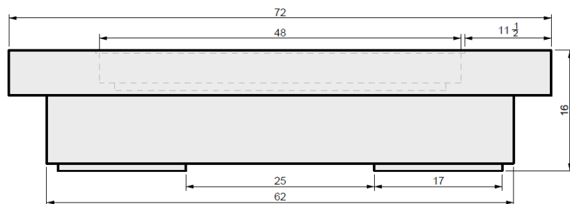
02 FRONT VIEW
