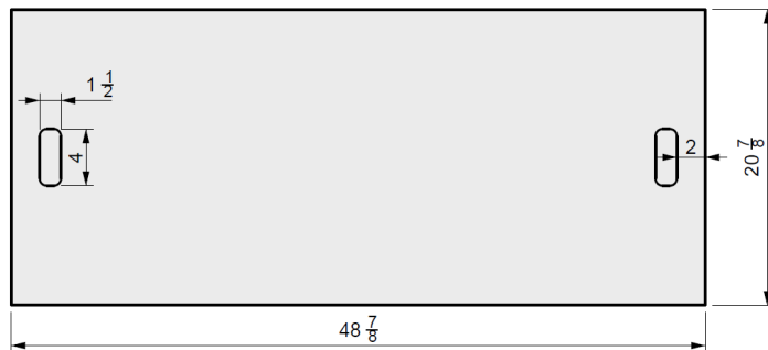
01 TOP VIEW
