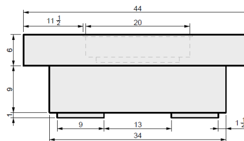
03 SIDE VIEW
