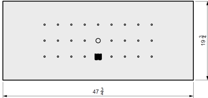
01 TOP VIEW
