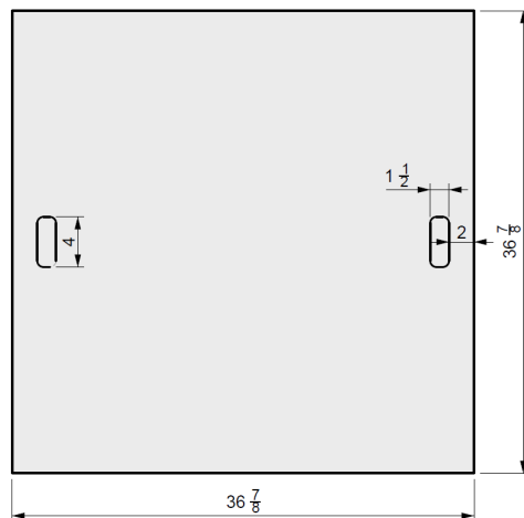
01 TOP VIEW
