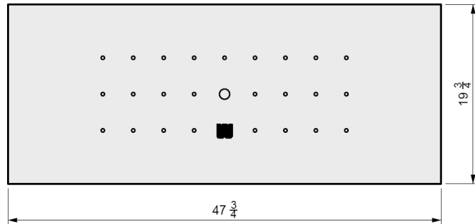
01 TOP VIEW
