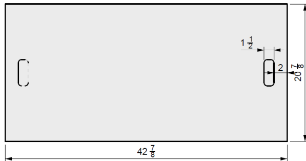
01 TOP VIEW
