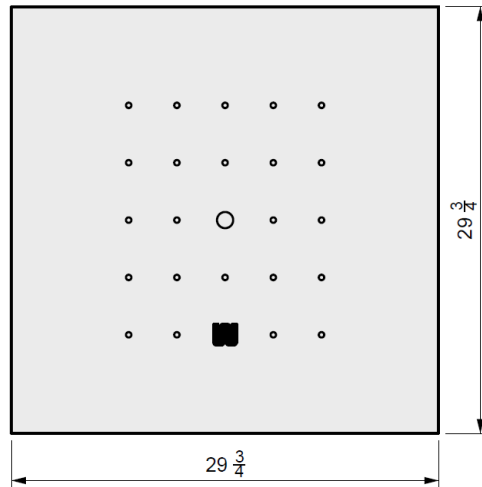
01 TOP VIEW
