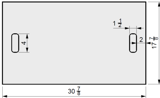
01 TOP VIEW
