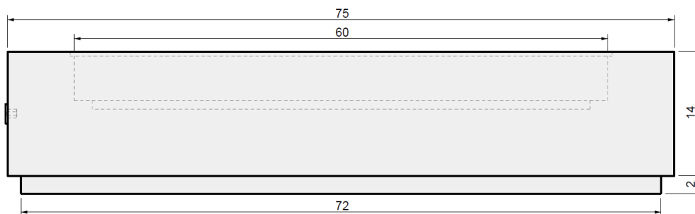
02 FRONT VIEW
