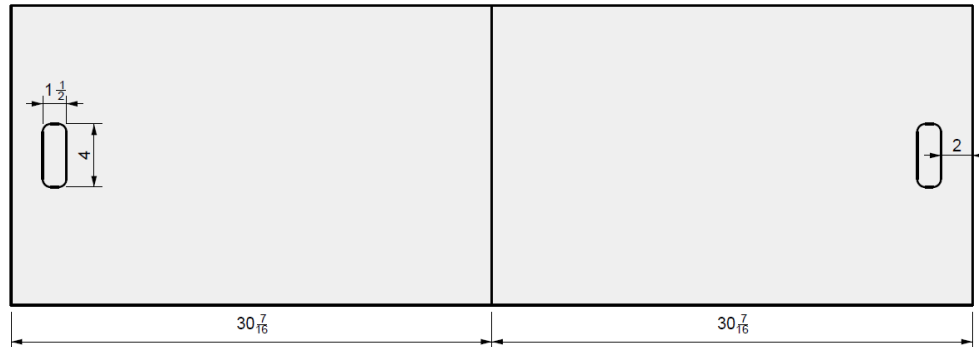
01 TOP VIEW
