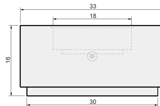
03 SIDE VIEW
