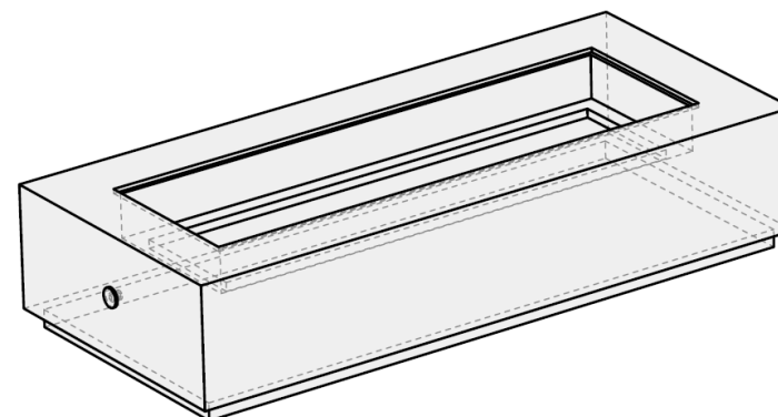
04 PERSPECTIVE
