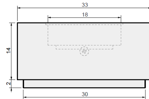
03 SIDE VIEW
