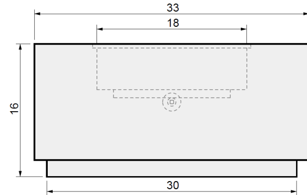
03 SIDE VIEW
