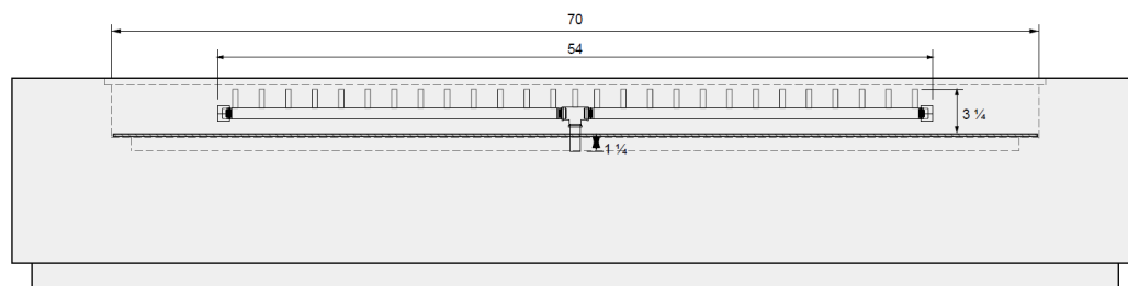
01 SIDE VIEW
