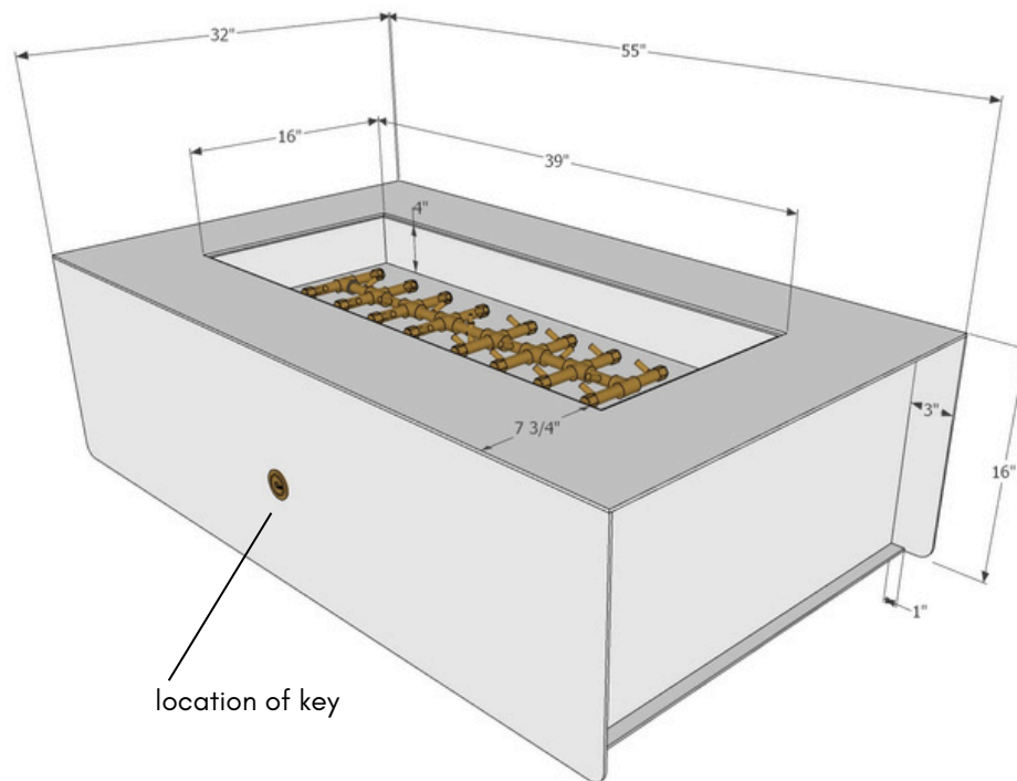
shown with upgraded burner
