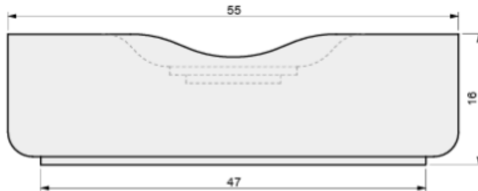
02 FRONT VIEW
