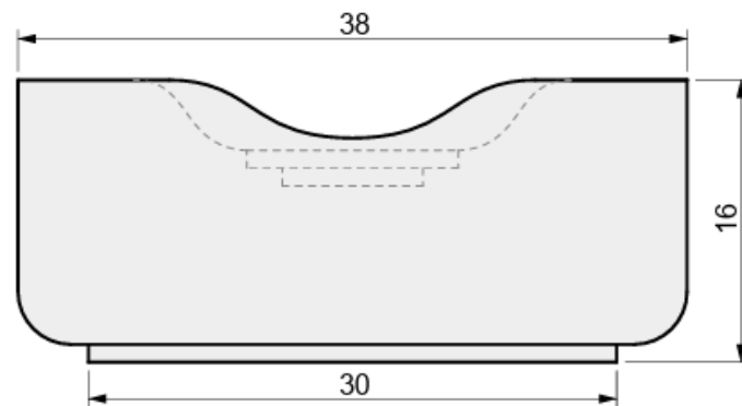
02 FRONT VIEW
