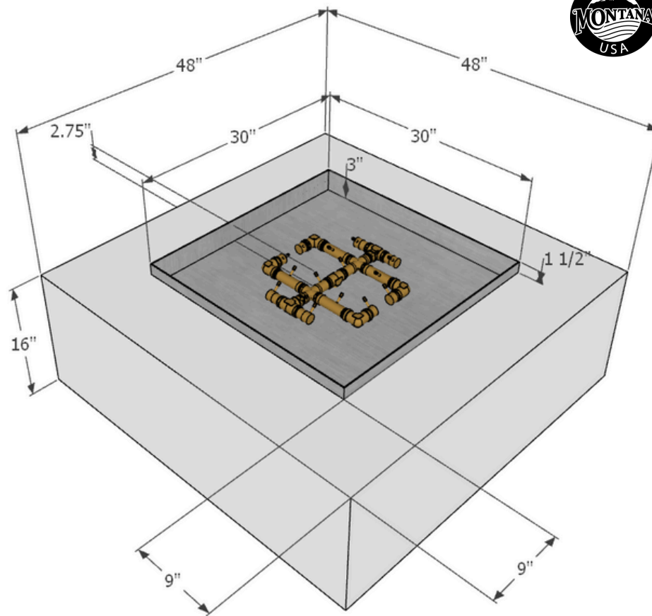
standard burner
