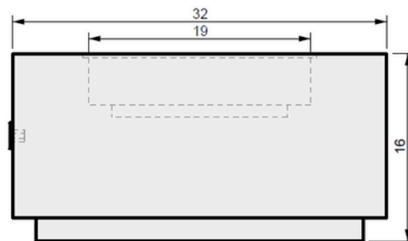
02 FRONT VIEW
