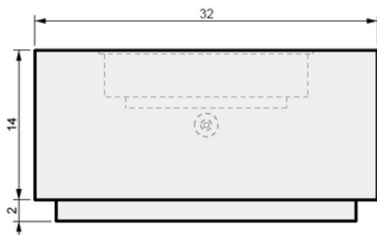
03 SIDE VIEW
