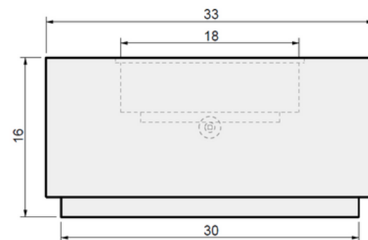
03 SIDE VIEW
