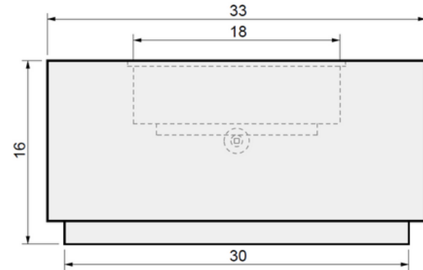
03 SIDE VIEW
