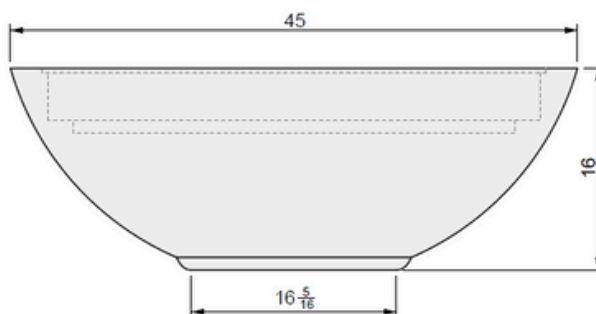
02 FRONT VIEW
