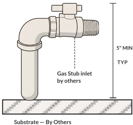
AAR.3 – 3 HARD LINE STUB UP
