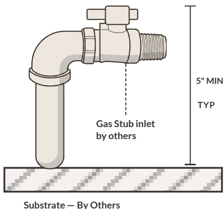
YSR.3 – 3 HARD LINE STUB UP
